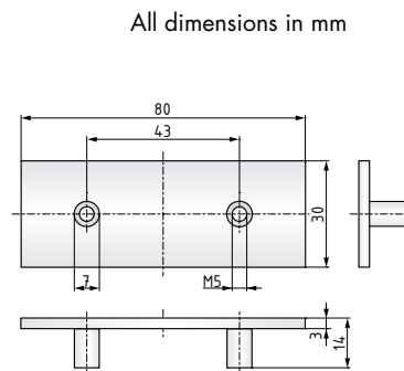
Counter plate for mounting bracket 205197 part no. 205468 (AISI 304)
