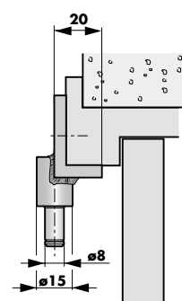
Mounting bracket TB 50x40x20 mm, pin 8 mm part no. 205263 (zinc-plated), 205258 (AISI 304)
