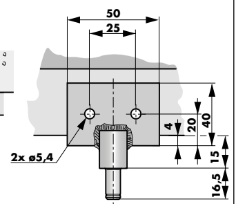
Mounting bracket TB 50x40x20 mm, pin 8 mm part no. 205263 (zinc-plated), 205258 (AISI 304)
