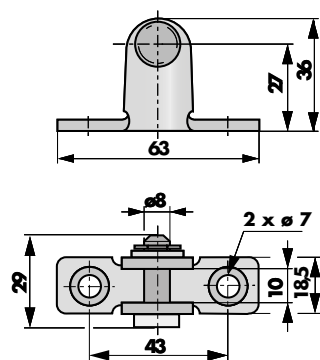
Mounting bracket part no. 205197 (zinc-plated), 205249 (AISI 304), 205455 (AISI 316)
