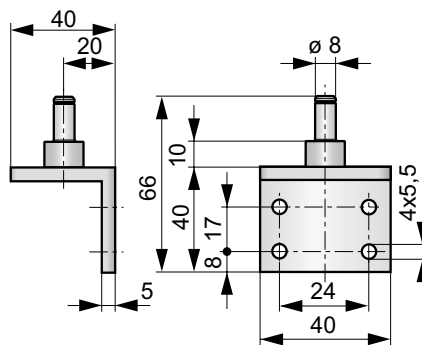
Mounting bracket TB 40x40x40 mm, pin 8 mm part no. 205262 (zinc-plated), 205282 (AISI 304), 205456 (AISI 316)
