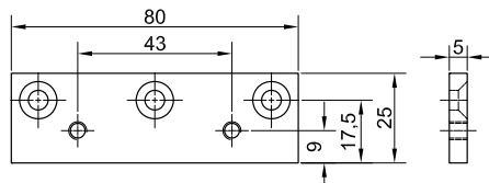
Mounting plate TB with 2 threaded holes M5 for mounting bracket 205197 part no. 205479 (AISI 304)
