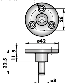
Mounting flange TB Ø 42 mm, pin 8 mm part no. 205261 (zinc-plated), 205281 (AISI 304)
