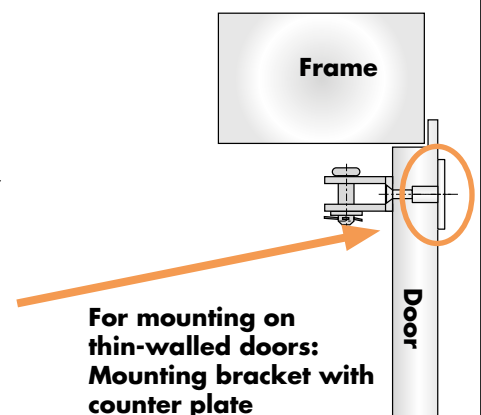
Counter plate for mounting bracket 205197 part no. 205468 (AISI 304)
