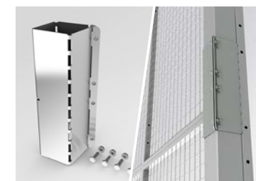
9 EXTENSION BRACKETS 80x80 A smart solution for taller Partitioning walls. Top fixing recommended when building beyond 4,400 mm.
