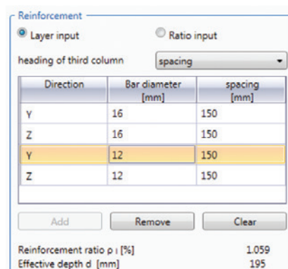
Example of multiple reinforcement layers
