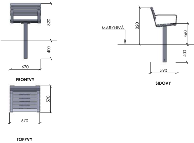
VRIDBAR STOL
