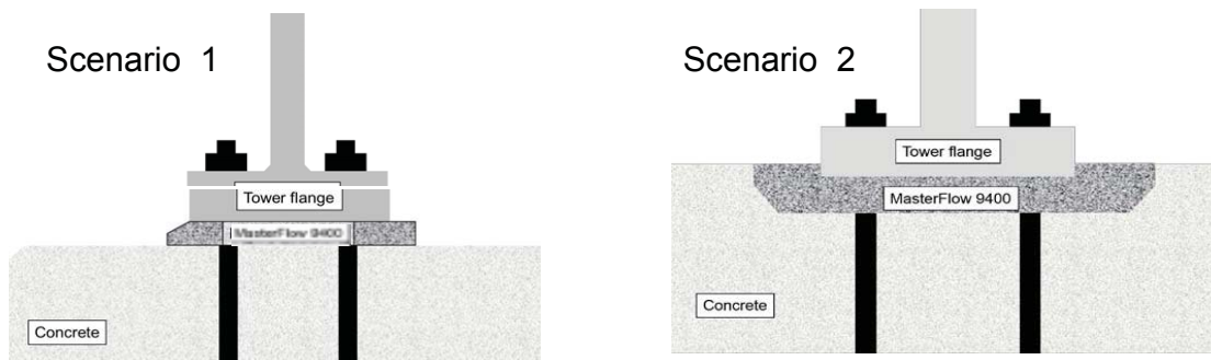
Situation after installation of tower base.
