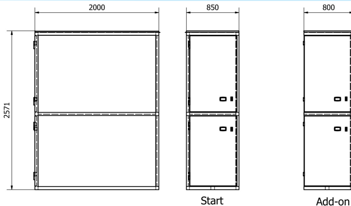
Side view
