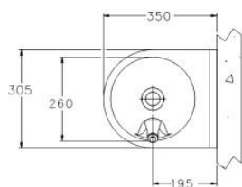
PLAN
