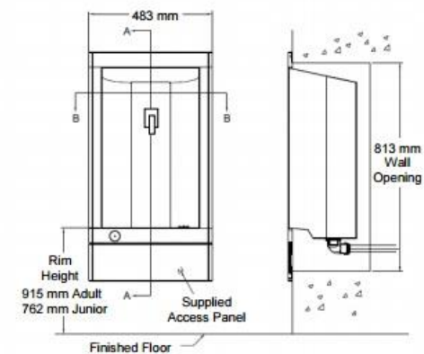
FRONT ELEVATION SIDE ELEVATION
