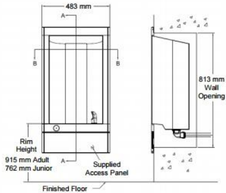
FRONT ELEVATION SIDE ELEVATION
