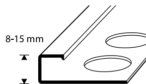
Kakelprofil H = 8 mm, 10 mm, 12 mm, 15 mm
