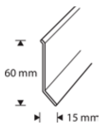
Socklar 60 x 15 mm
