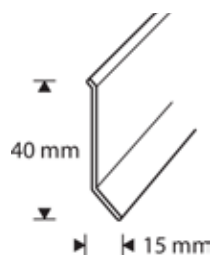
Socklar 40 x 15 mm
