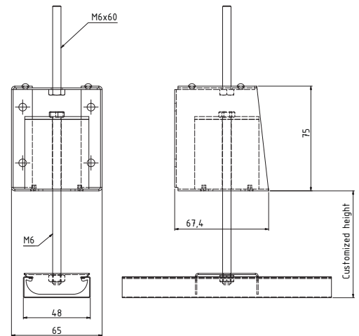
VT-MCH Top-mounted With click-on system
