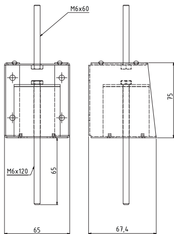
VT-MCH Top-mounted
