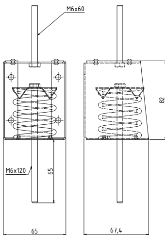
VT-MSH Top-mounted
