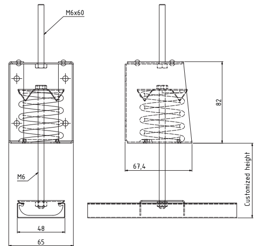
VT-MSH Top-mounted With click-on system
